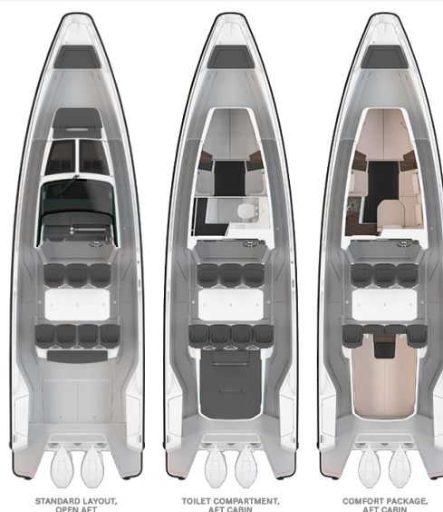
STANDARD LAYOUT, OPEN AFT
